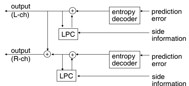
Fig. 1. Decoding process of reference predictive coding system with simple inter-channel prediction.
