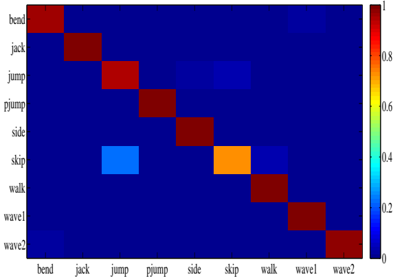
Fig. 3. Confusion matrix on the Weizmann dataset with FTLE-HoG + \Lambda_{arcL} -HoG features of cell size 16 (Mean accuracy: 97.55).
