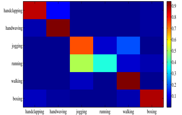
Fig. 4. Confusion matrix on the KTH dataset with FTLE-HoG + \Lambda_{arcL} -HoG features of cell size 8 (Mean accuracy: 87.84).
