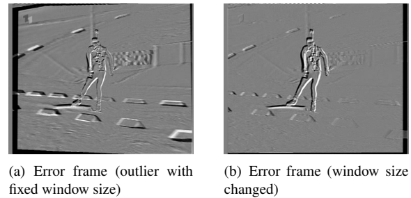
Fig. 4. Comparison of a fixed window size and variable window size at the outlier case (frame 94, “Biathlon” sequence)
